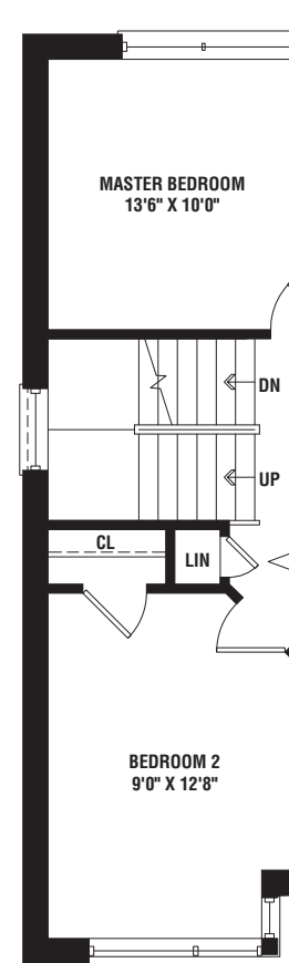
PARTIAL THIRD FLOOR ELEV. 'B' INTERIOR END CONDITION
