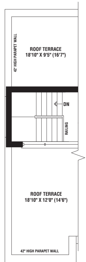
PARTIAL MEZZANINE ELEV. 'B' INTERIOR END CONDITION
