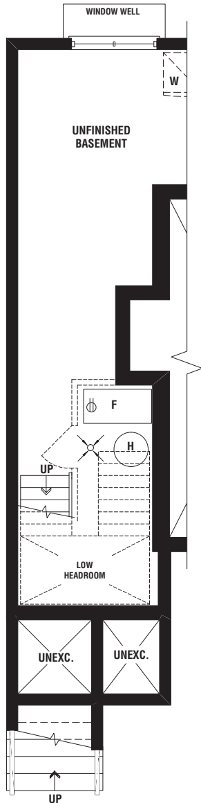
PARTIAL BASEMENT FLOOR ELEV. 'B' INTERIOR END CONDITION
