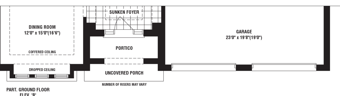
PART. GROUND FLOOR ELEV. 'B'
