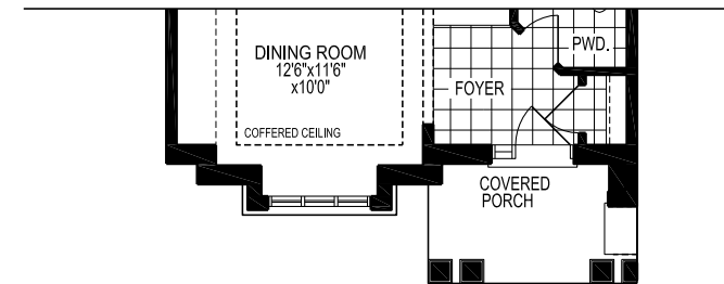
GROUND FLOOR PLAN 'B'
