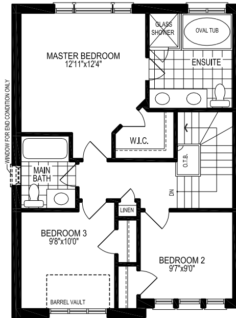
SECOND FLOOR PLAN 'A'
