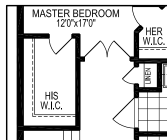
PART-SECOND FLOOR PLAN W/ OPT. HIS & HERS W.I.C.
