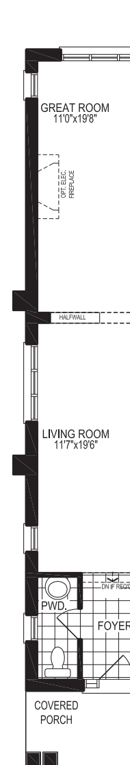
PART. GROUND FLOOR PLAN CORNER UPGRADE
