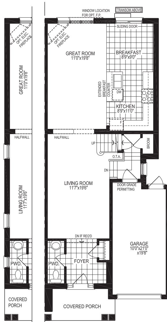
GROUND FLOOR PLAN END CONDITION
