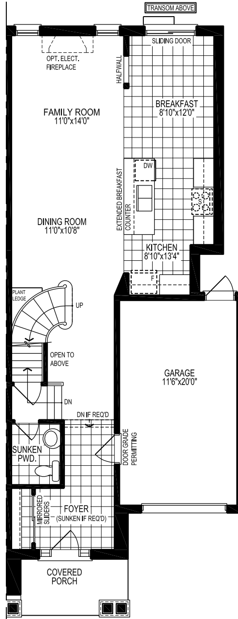
GROUND FLOOR PLAN END CONDITION
