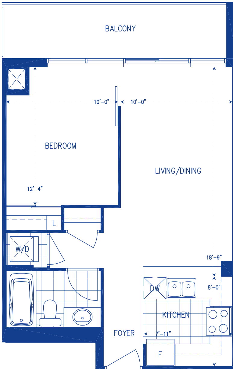
10TH FLOOR PLAN
