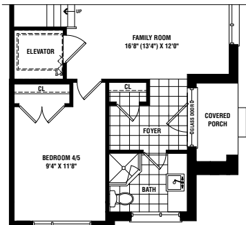
GROUND FLOOR ELEV. 'A'
