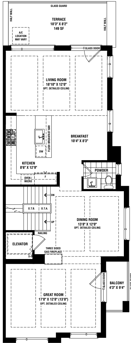
MAIN FLOOR ELEV. 'A'
